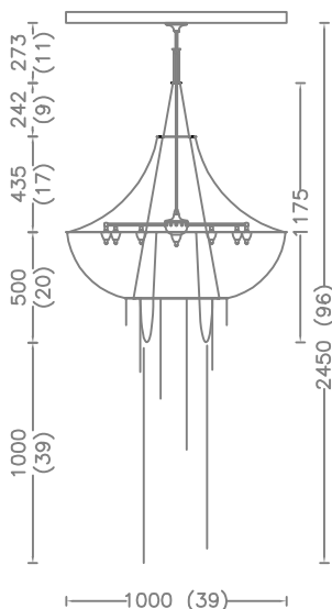
FOLC-1000 - CHANDELIER
