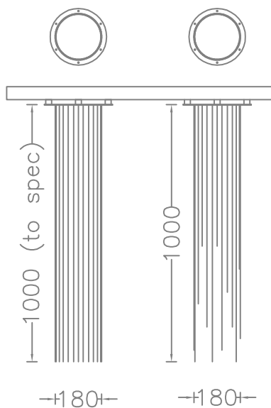
DOWNLIGHTER RETROFIT DR-180
