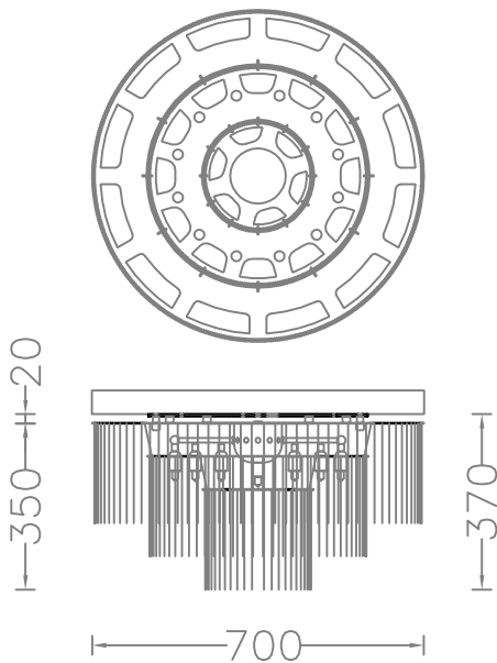
3-TIER-700-CEILING Chandelier
